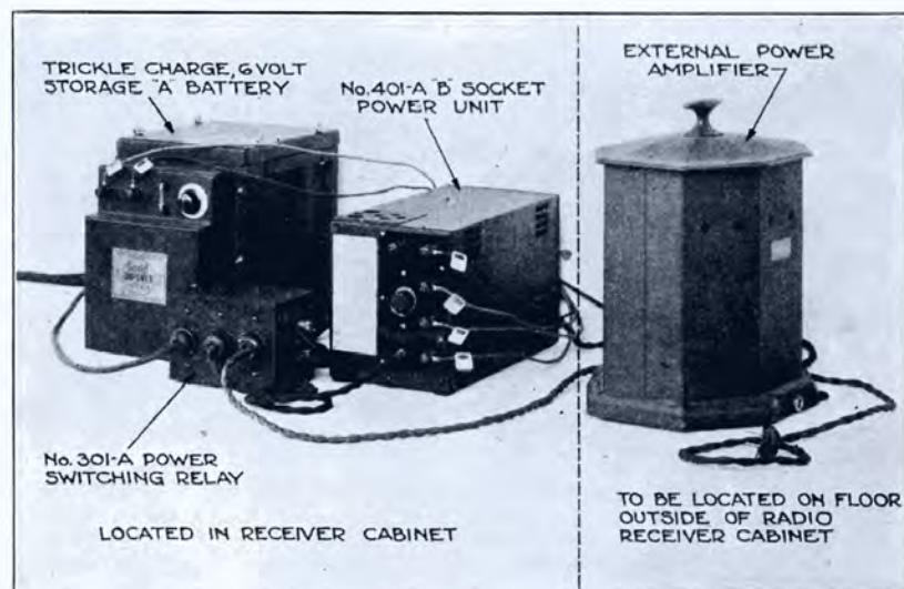
Fig. 30—Arrangement of Current Supply Apparatus for Circuit Fig. 8
