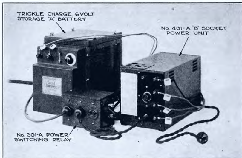
Figs. 28 and 29—Arrangement of Current Supply Apparatus for Circuits Figs. 6 and 7
