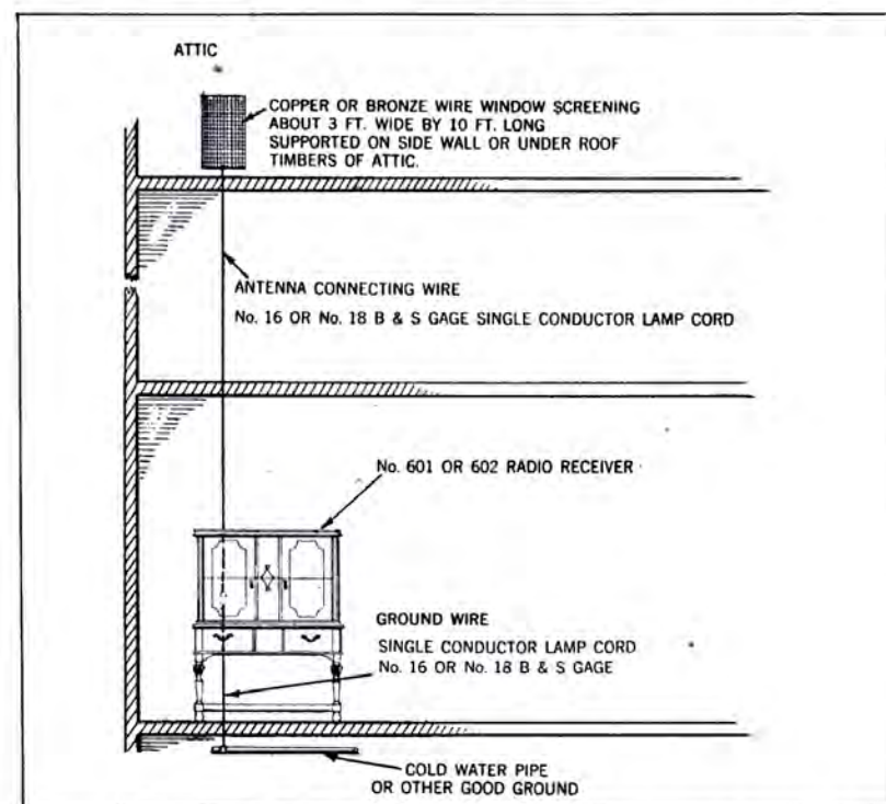
Fig. 38—Attic Antenna, using window screening for Pick-up
