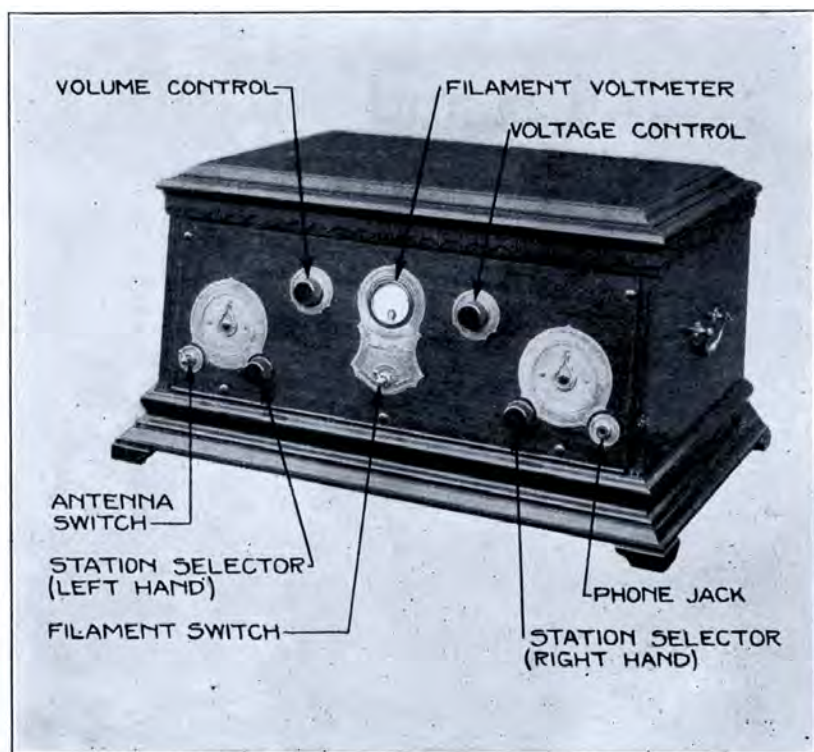
Fig. 1—Location of Controls for the No. 601-B "Treasure Chest" Radio Receiver. The same Controls are provided for the No. 602-B "Art Console" Receiver
