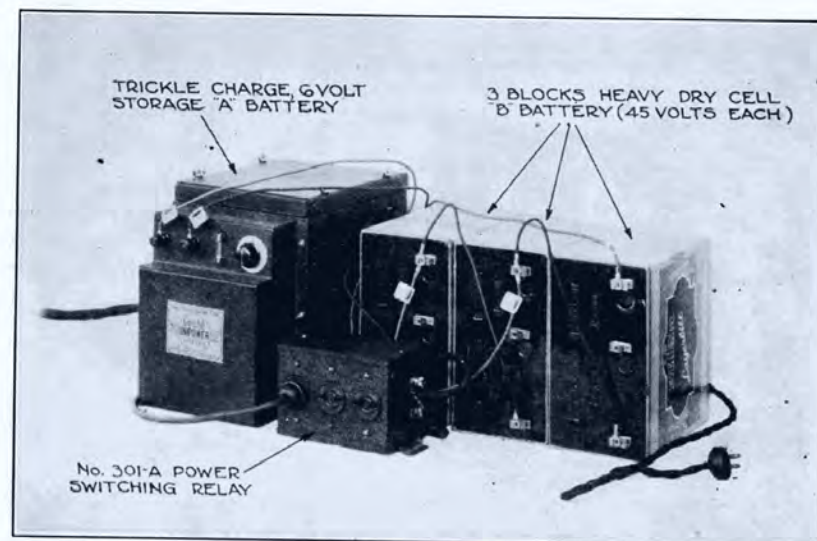
Fig. 26—Arrangement of Current Supply Apparatus for Circuit Fig. 4
