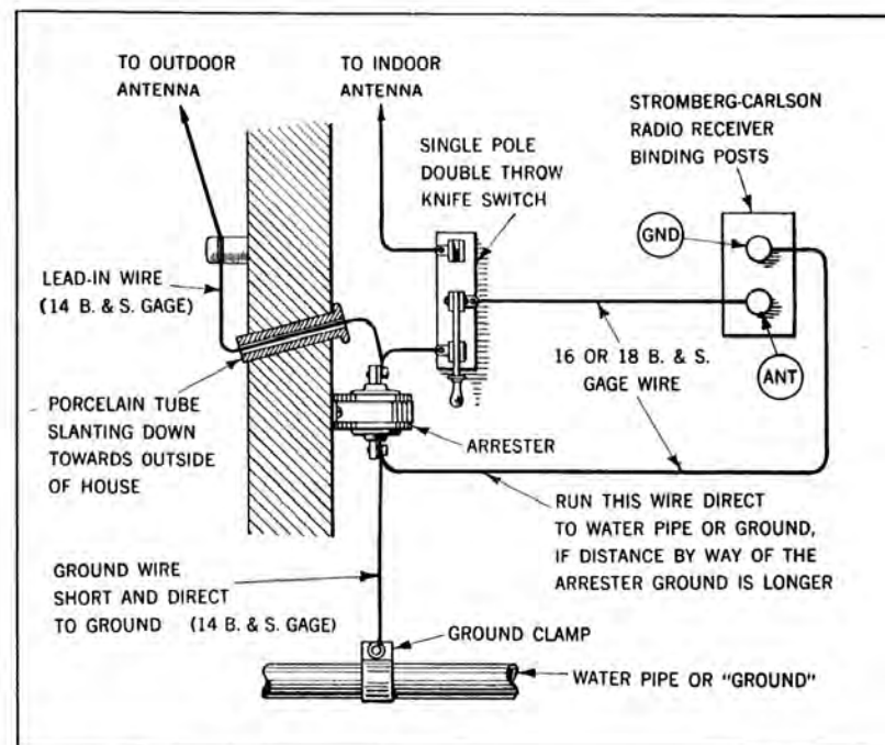
Fig. 41—Inside Ground for Arrester and Receiver, used when both Arrester and Ground are located close together. This allows a long outdoor or a short indoor Antenna to be used as desired
