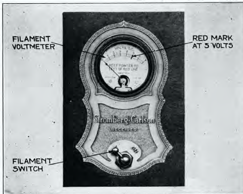
Fig. 18—Filament Voltmeter and Filament Switch
