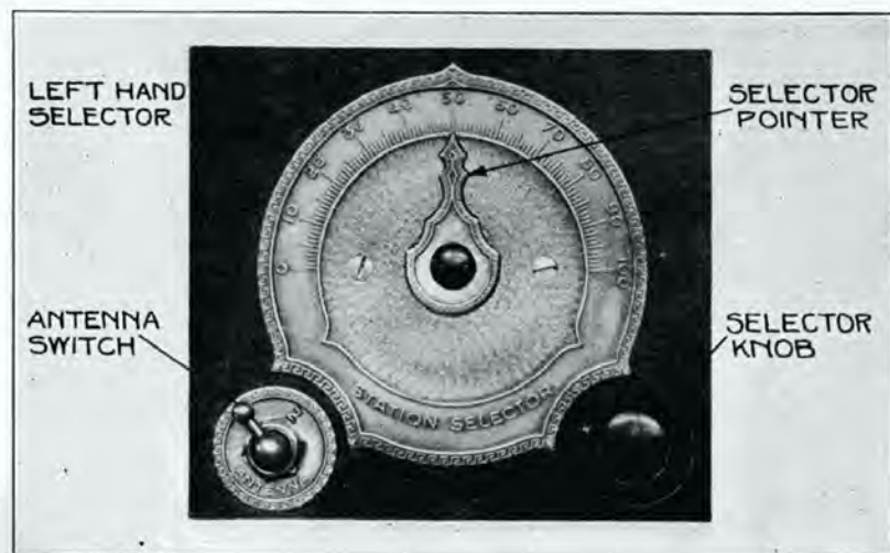
Fig. 16—Left Hand Station Selector with Operating Knob at right and Antenna Coupling Key at the left
