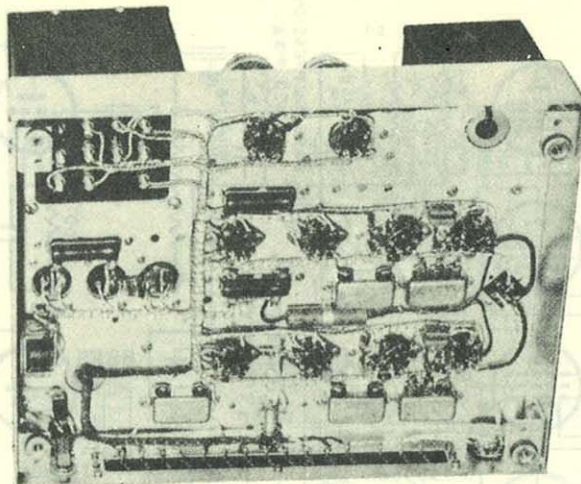
Bottom View of No. 27 Amplifier Brief Specifications
